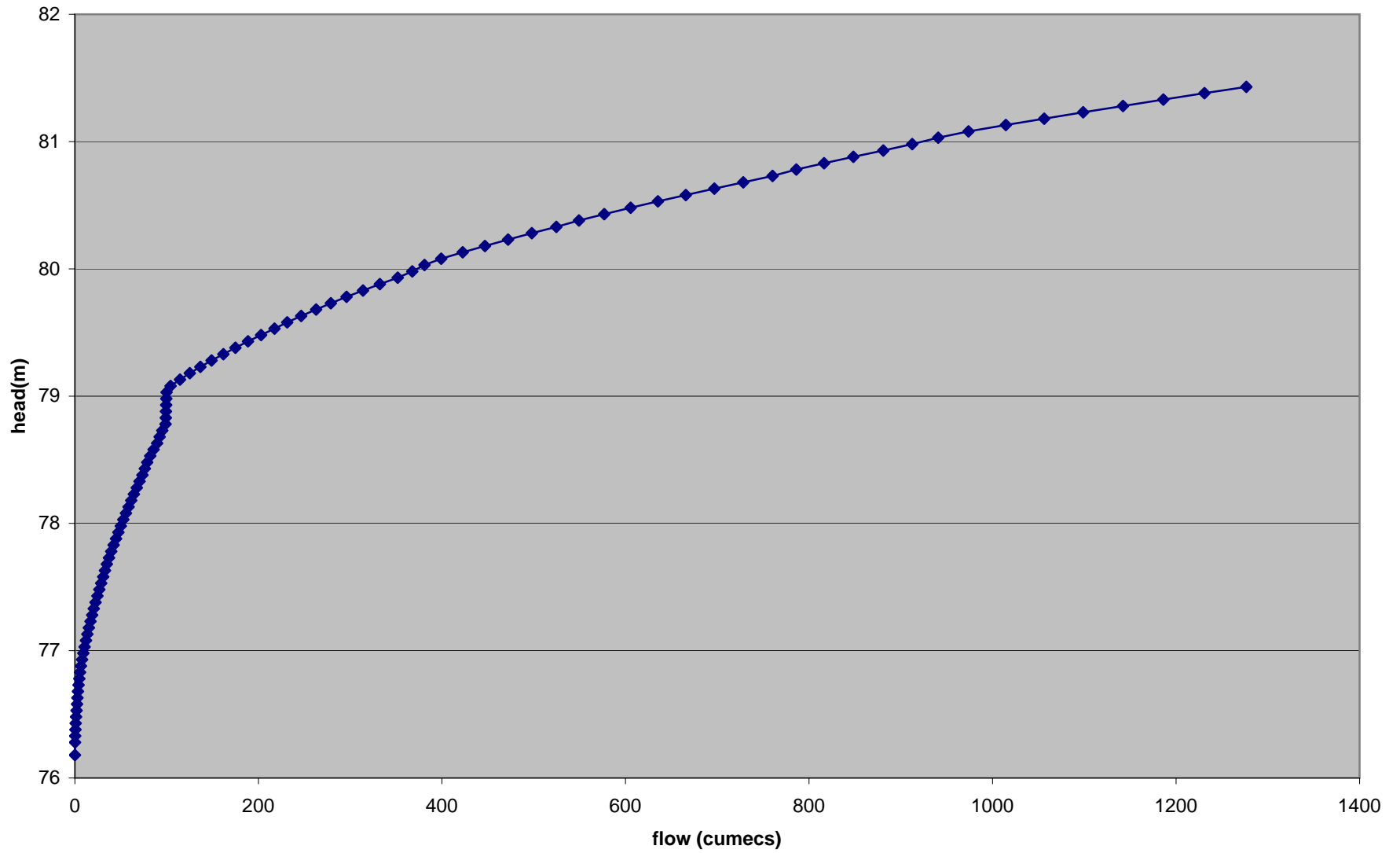
Downstream boundary rating curve
