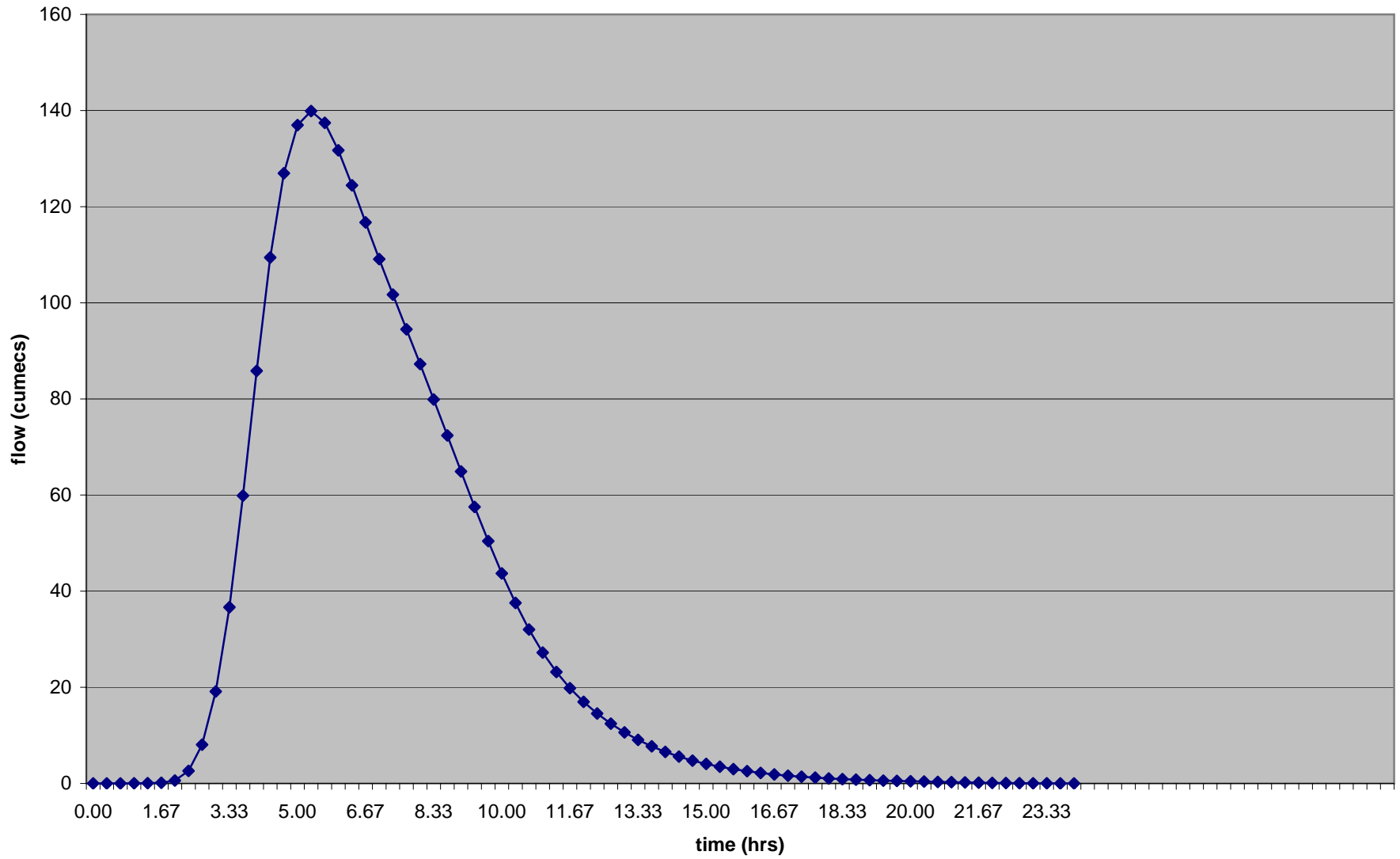
Q100( + 20% increase in flow) Upstream boundary condition
