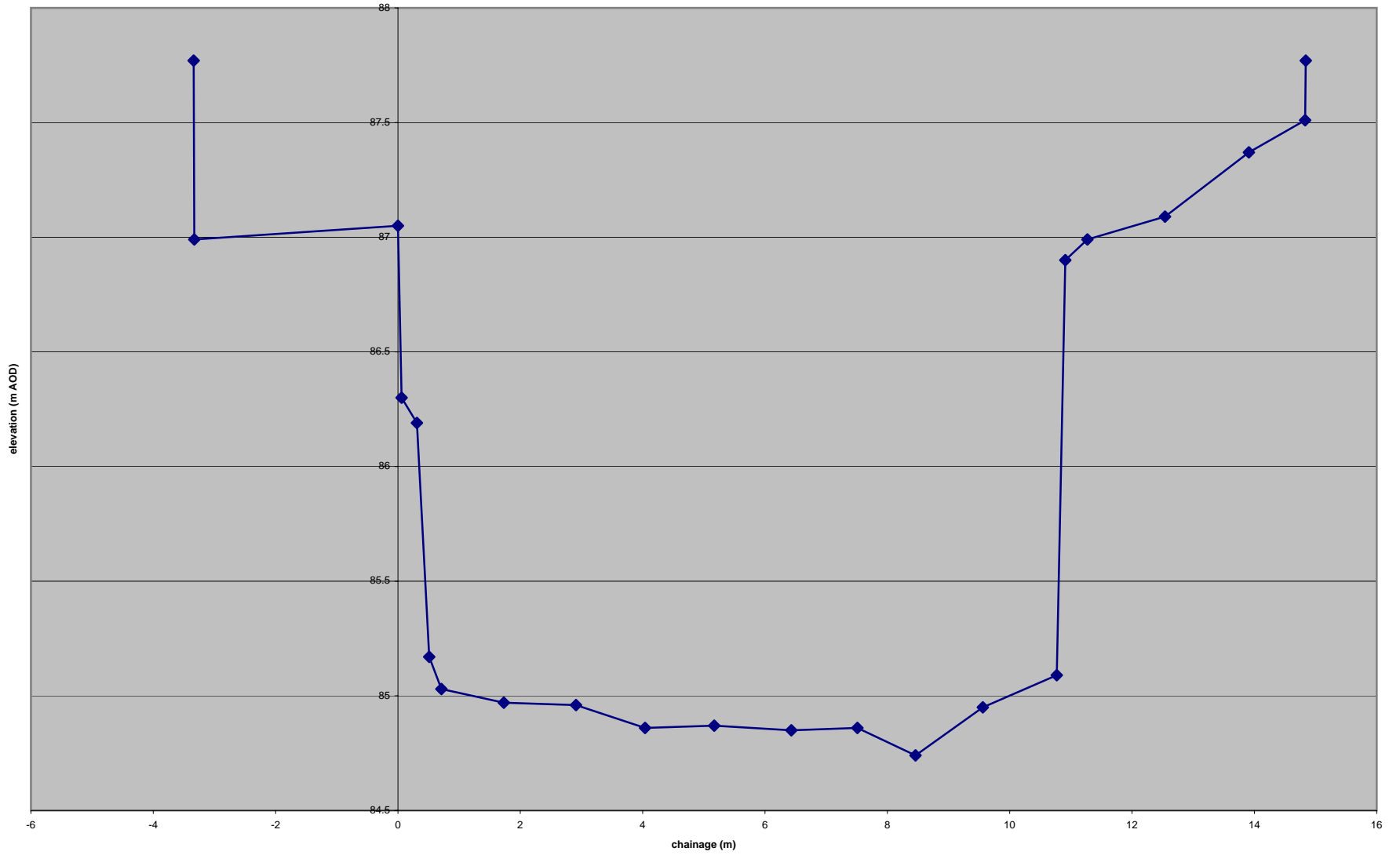
cross section ponty1.3231
