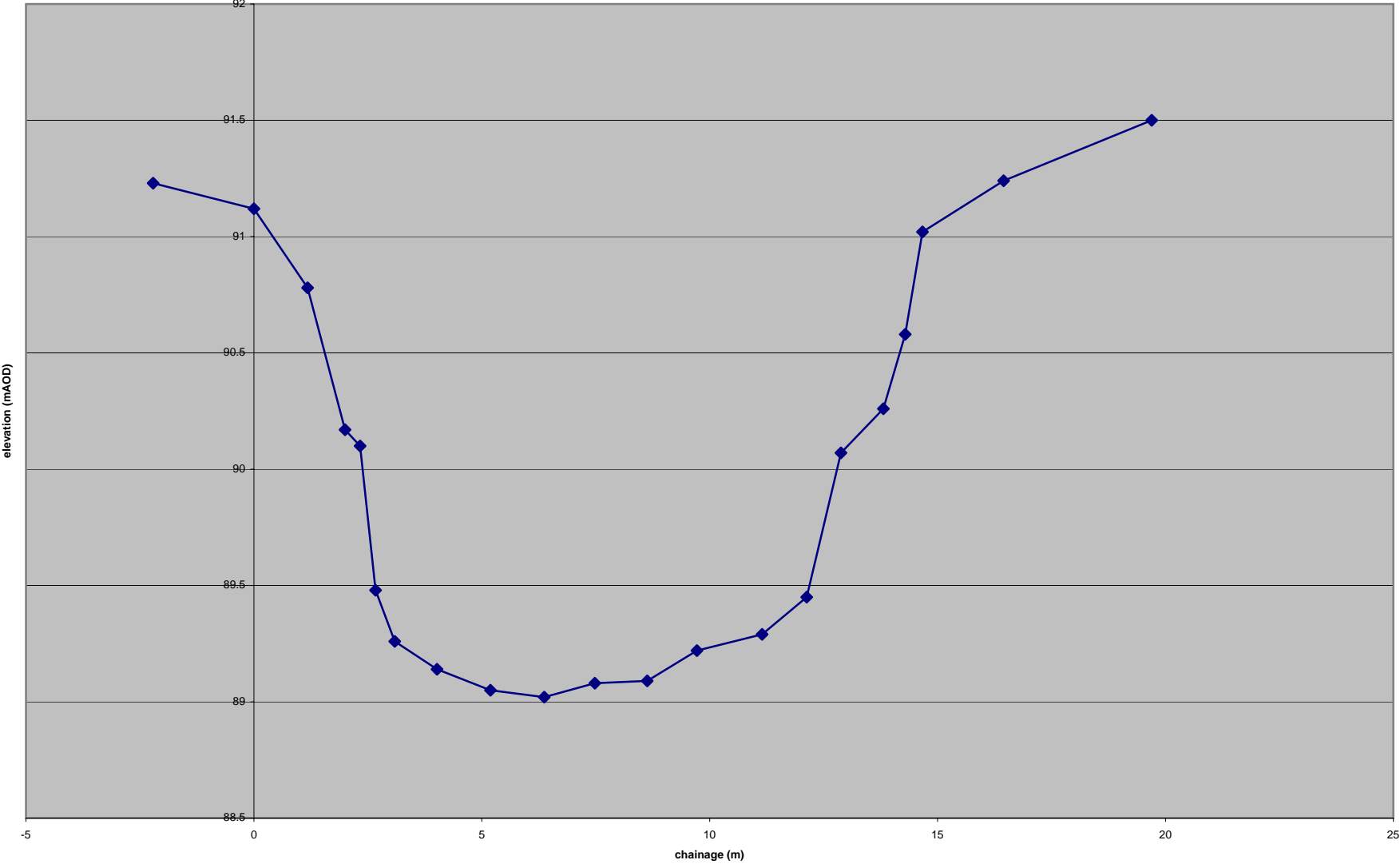
cross section ponty1.38
